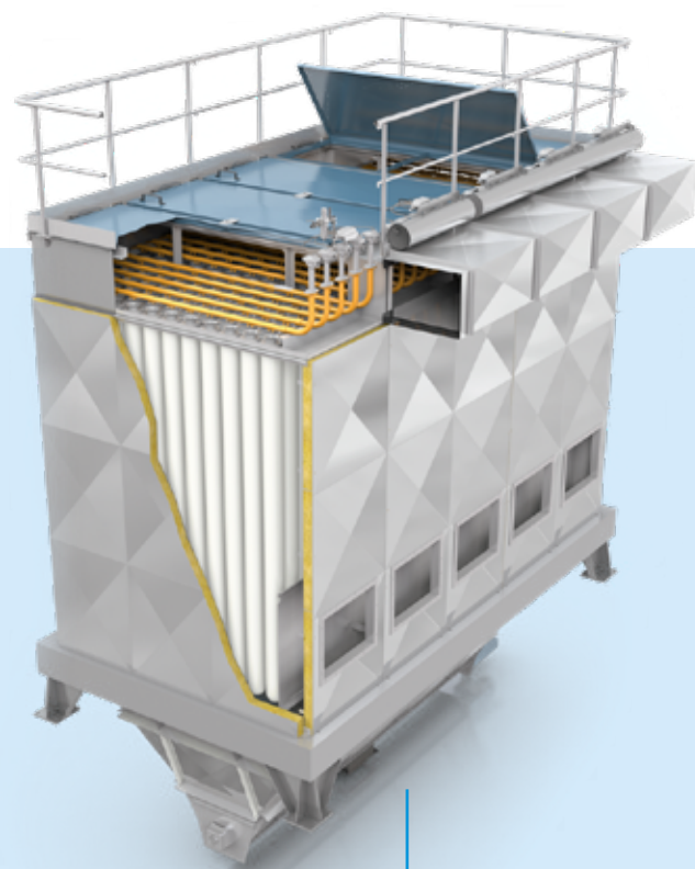
SCHEUCH HOT GAS FILTER / CATALYTIC HOT GAS FILTER
