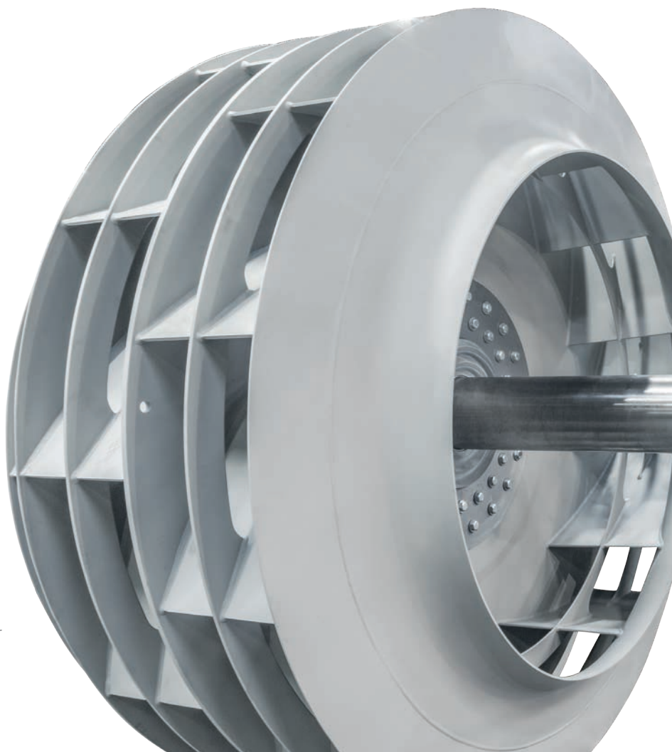
Impeller for double-flow radial fan
